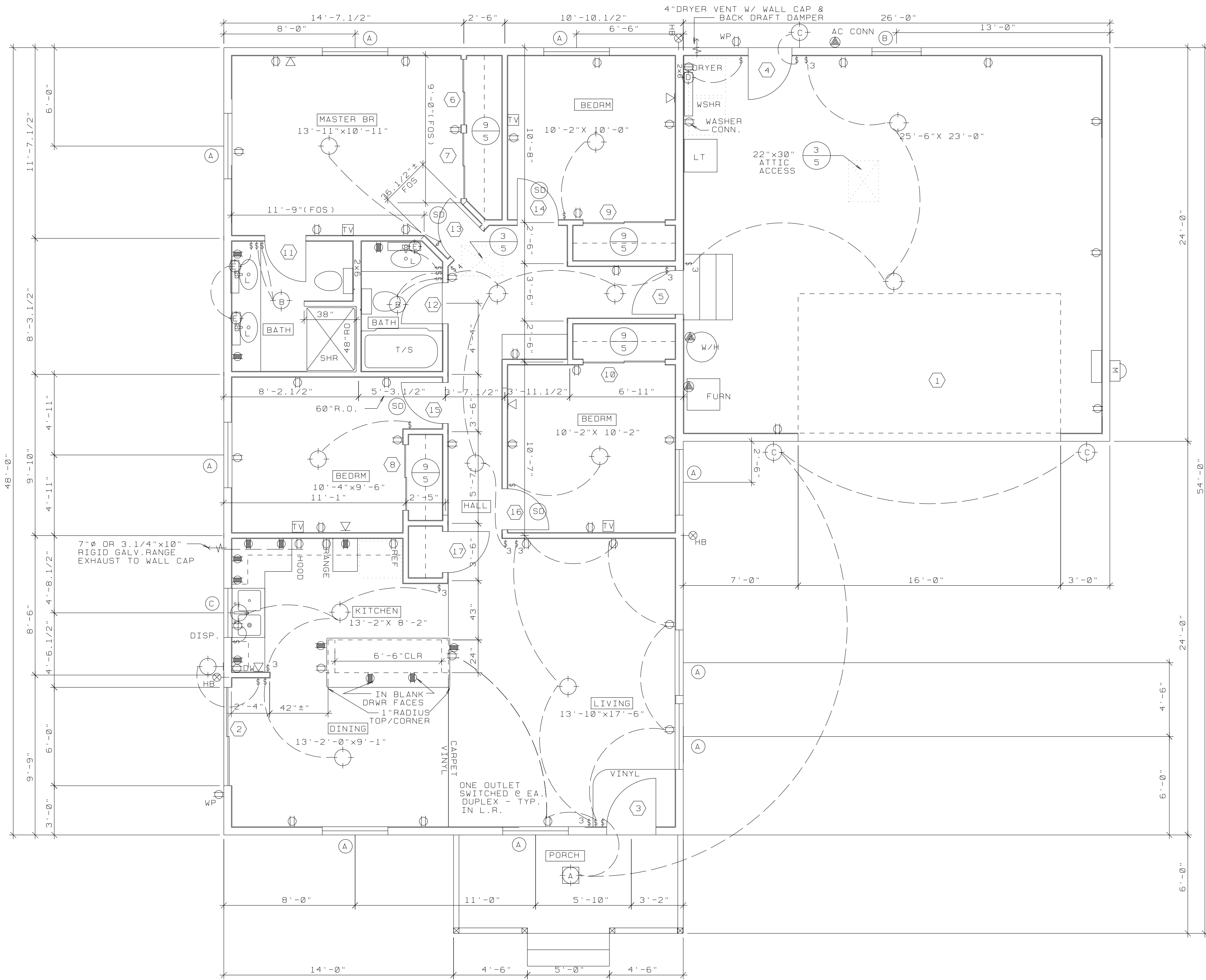
FLOOR PLAN 4 BEDROOM 1344 SF UNLESS NOTED OTHERWISE ALL WALLS 2x4 @ 16" OC INTERIOR 2x6 @ 16" EXTERIOR. 1/4"=1'-0" A6009-1344SF-4BR-RA
